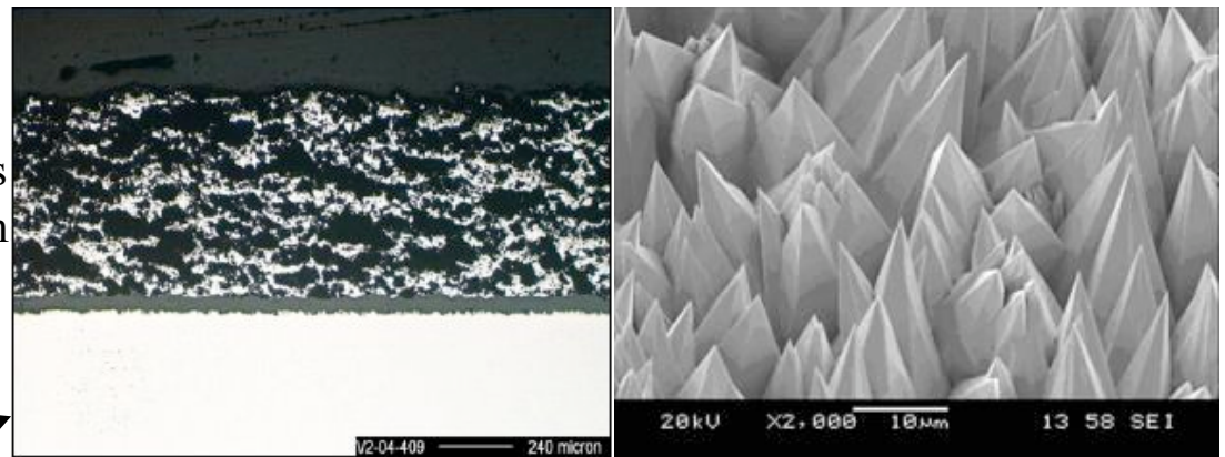
Micrographs of candidate lithium-retaining surfaces
