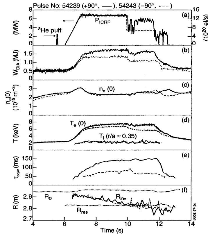
FIG. 1. Overview of two 3.45T/1.8 MA JET ^4\text{He} discharges with ^3\text{He} minority heating using +90° and -90° phasings.
